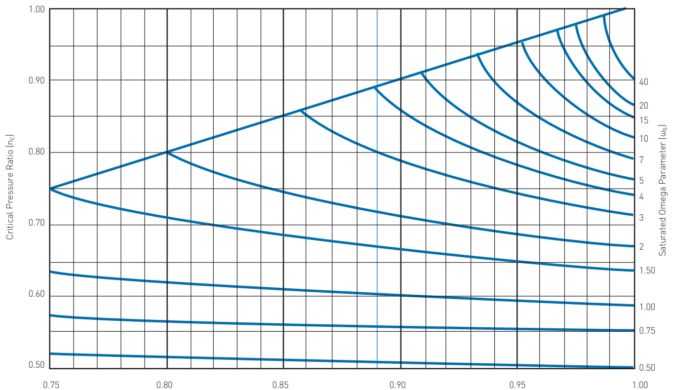
FIGURE 6-3 Saturated Pressure Ratio ( \eta_s ) Critical Pressure Ratio for Low Subcooled Region Flashing Liquids
