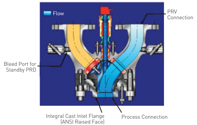
FIGURE 3-5 Safety Selector Valve
