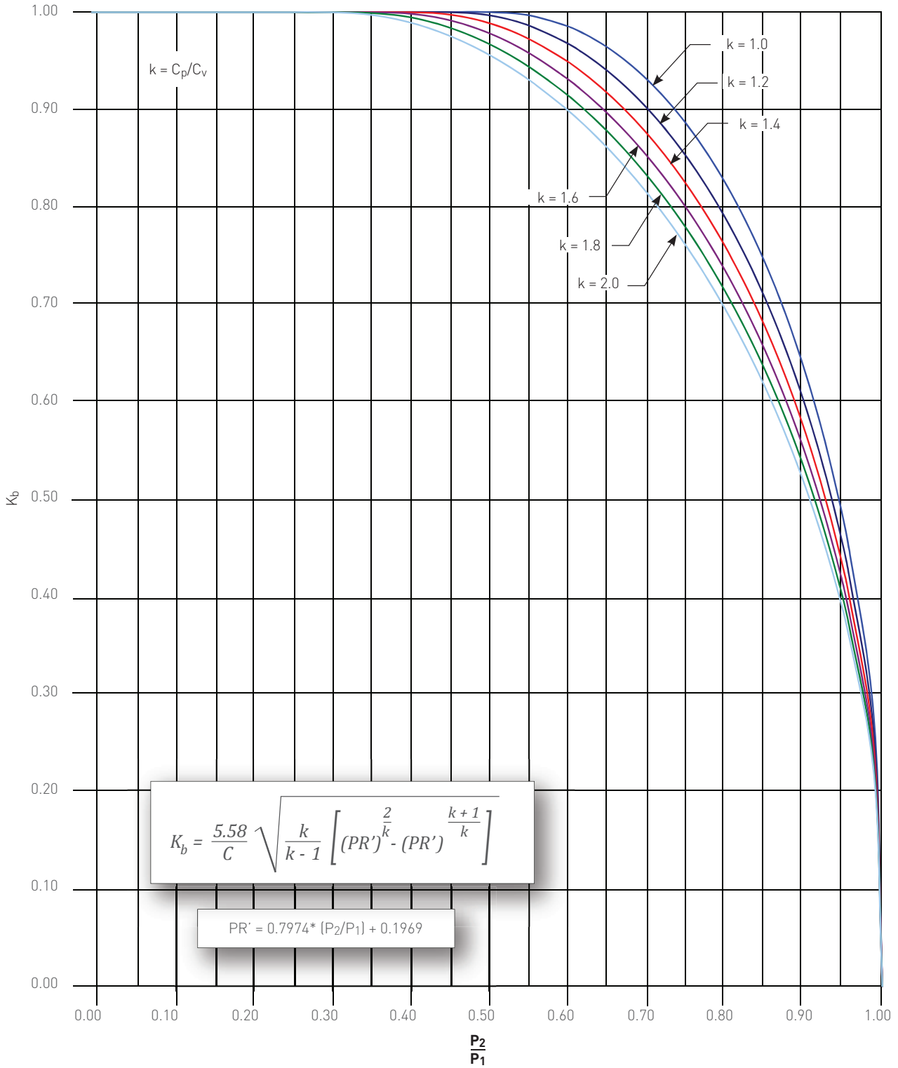
FIGURE 8-21 Anderson Greenwood Series 81P (-8 Orifice Only) Balanced Piston Direct Spring PRV Back Pressure Correction Factor ( K_b ) - Gas Service
