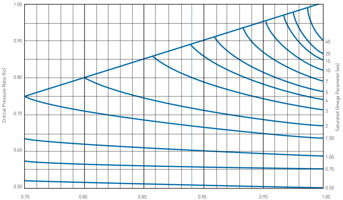
FIGURE 5-4 Saturated Pressure Ratio ( \eta_s ) Critical Pressure Ratio for Low Subcooled Region Flashing Liquids
