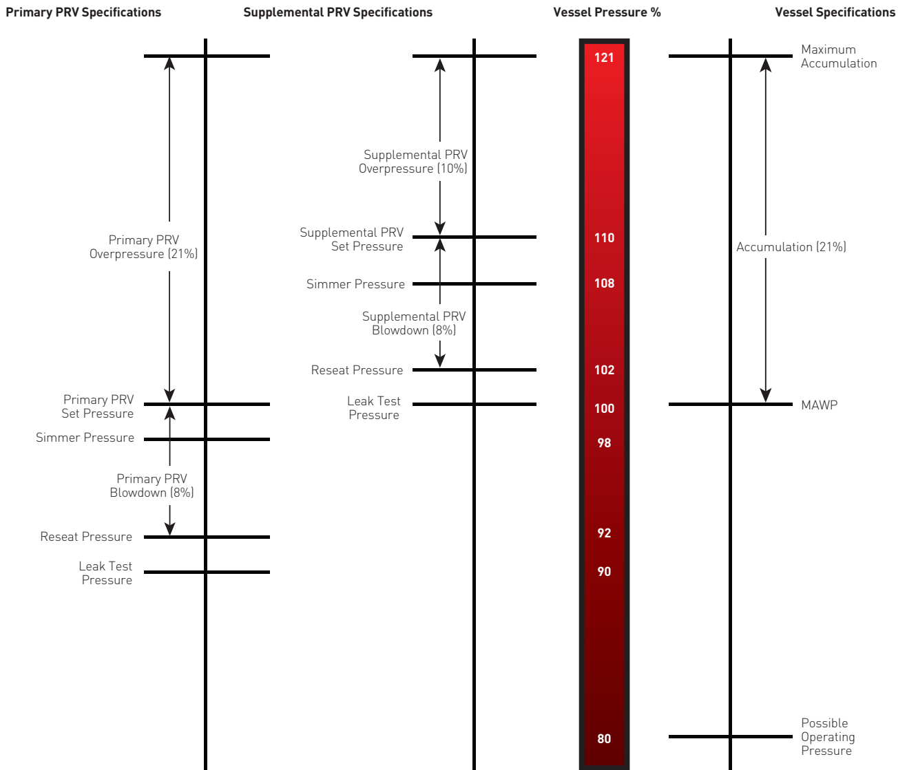
FIGURE 3-11 Typical Section VIII Multiple Valve (Non-Fire Case) Installation
