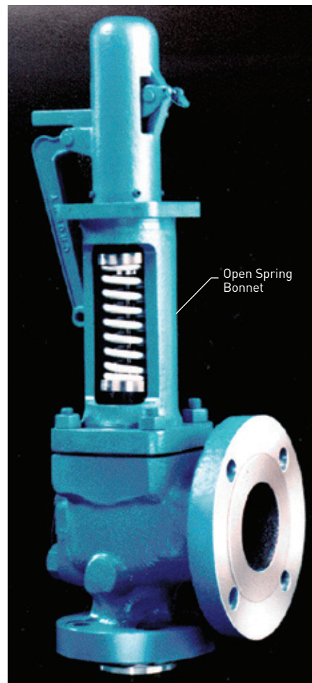
FIGURE 4-15 Open Bonnet Direct Spring PRV
