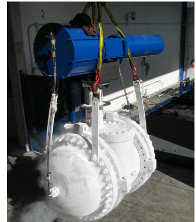
42" ASME Class 150 VANESSA Buttweld Top Entry upon cryogenic test
