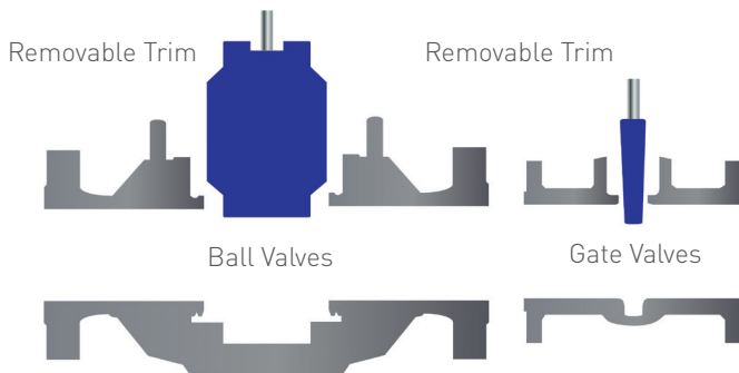
Other Top Entry Designs With Removable Trim
